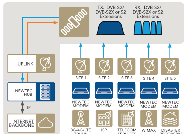
Point-to-multipoint
